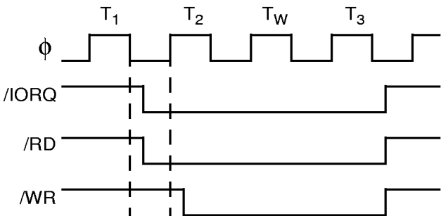
Figure 11. I/O Read and Write Cycles with IOC = 1
