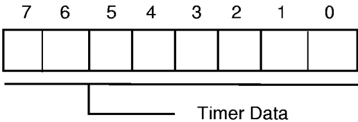
Figure 48. Timer Data Register 1L
