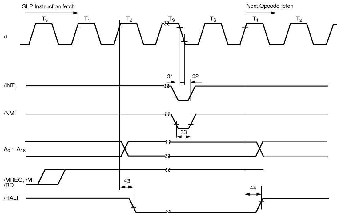
Figure 28. SLP Execution Cycle
