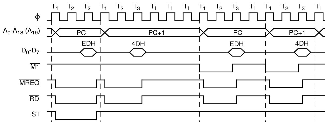
Figure 9. RETI Instruction Sequence with MIE=0
