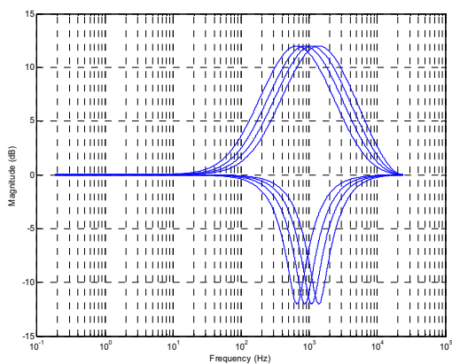
Figure 46 EQ Band 3 – Peak Filter Centre Frequencies, EQ3
