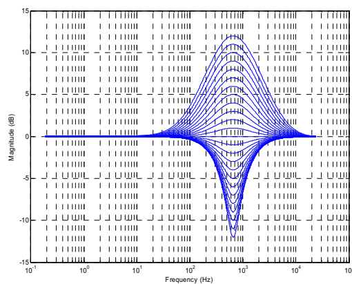
Figure 47 EQ Band 3 – Peak Filter Gains for Lowest Cut-off Frequency, EQ3BW=0
