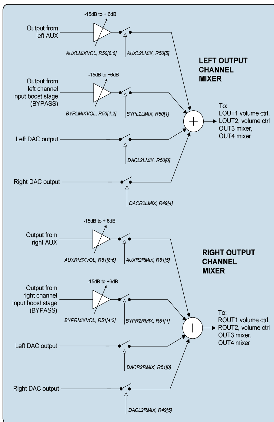
Figure 14 Left/Right Output Channel Mixers
