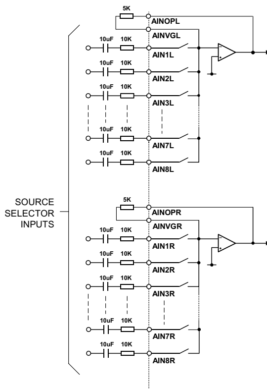
Figure 19 ADC Input Multiplexor Configuration
