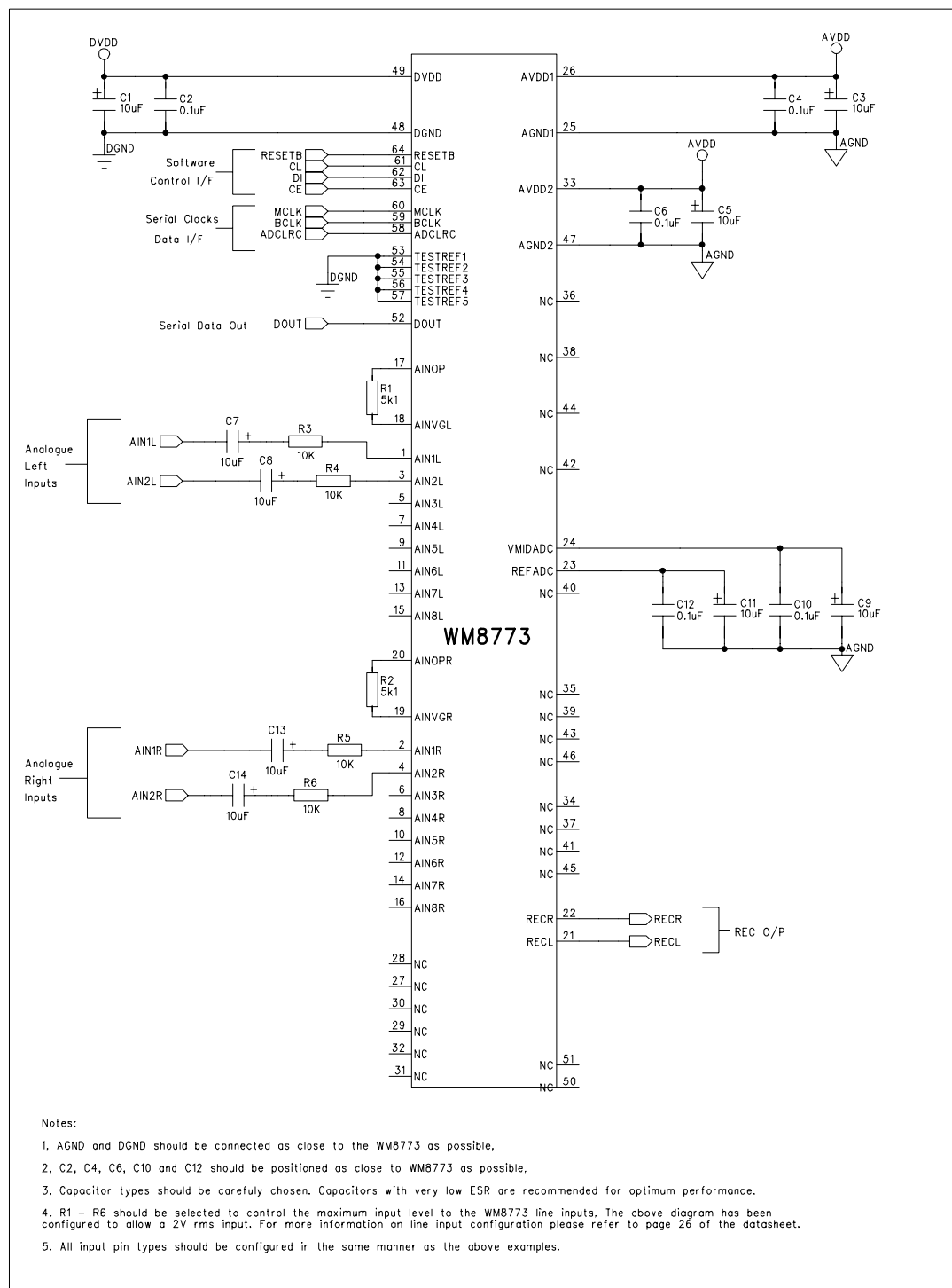
Figure 18 External Component Diagram
