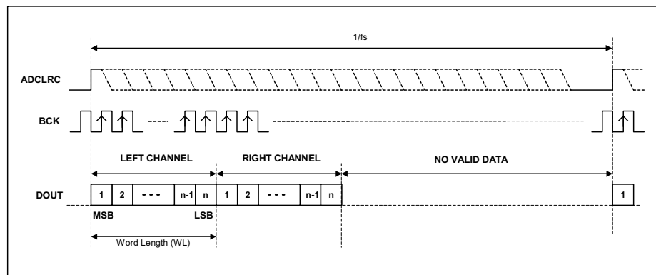
Figure 13 DSP Late Mode Timing Diagram – ADC Data Output
