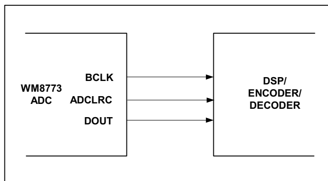
Figure 8 Master Mode
