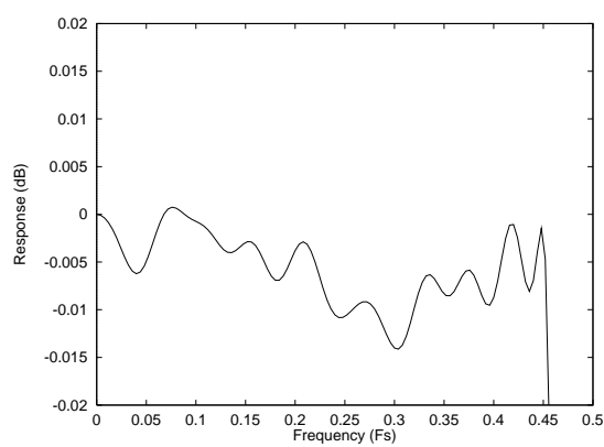
Figure 16 ADC Digital Filter Ripple
