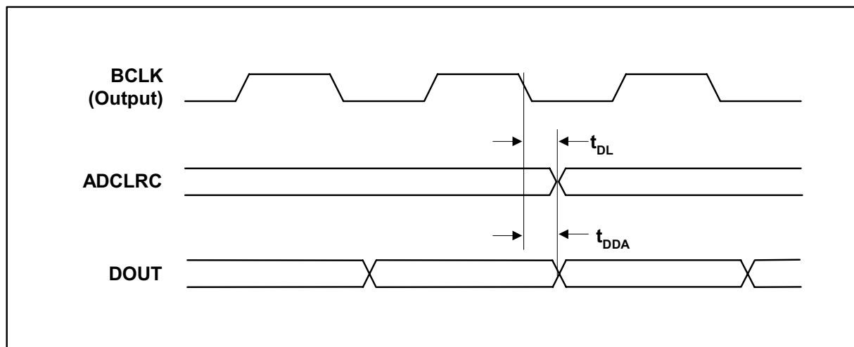
Figure 3 Digital Audio Data Timing – Master Mode
