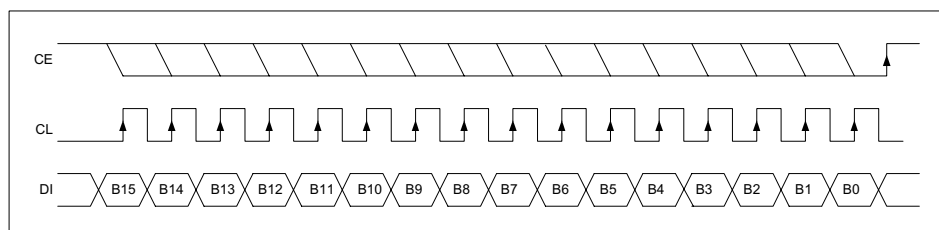
Figure 14 3-wire SPI Compatible Interface
