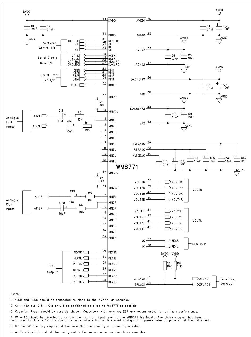
Figure 36 Recommended External Component Diagram
