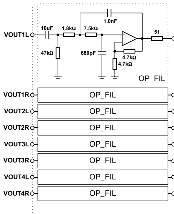
Figure 37 Recommended Post DAC Filter Circuit
