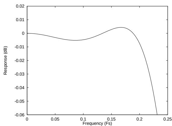
Figure 47 ADC Digital Filter Ripple –Type 2
