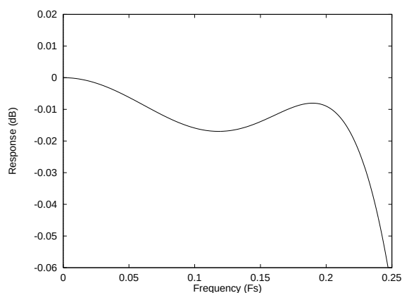
Figure 49 ADC Digital Filter Ripple –Type 3
