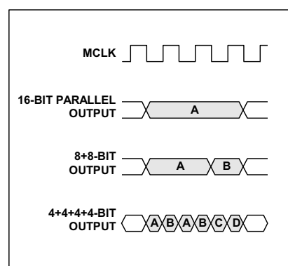
Figure 14 Output Data Formats (Mode 3)
