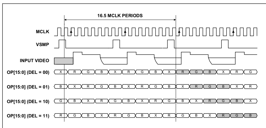
Figure 25 Mode 5 Operation (MCLK:VSMP Ratio = 8:1)
