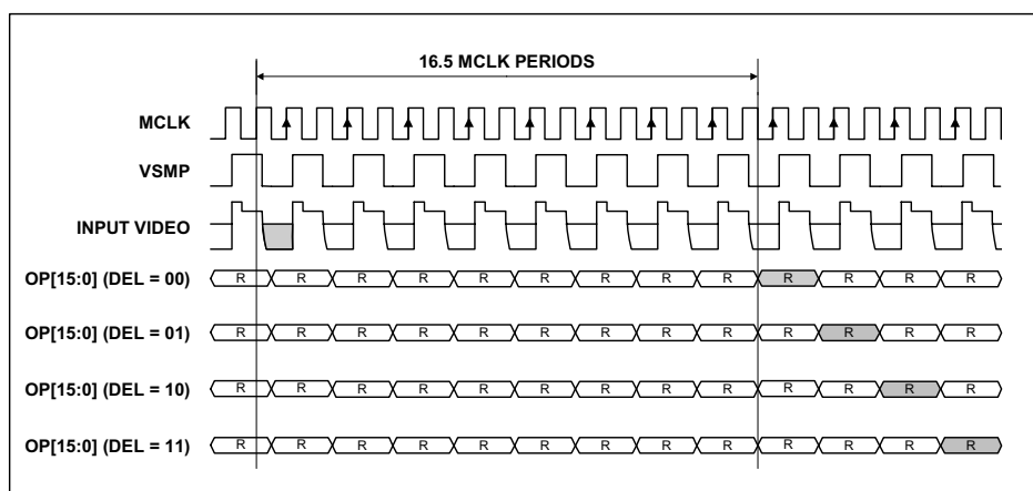
Figure 24 Mode 4 Operation
