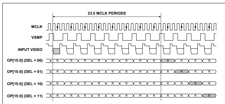
Figure 23 Mode 3 Operation
