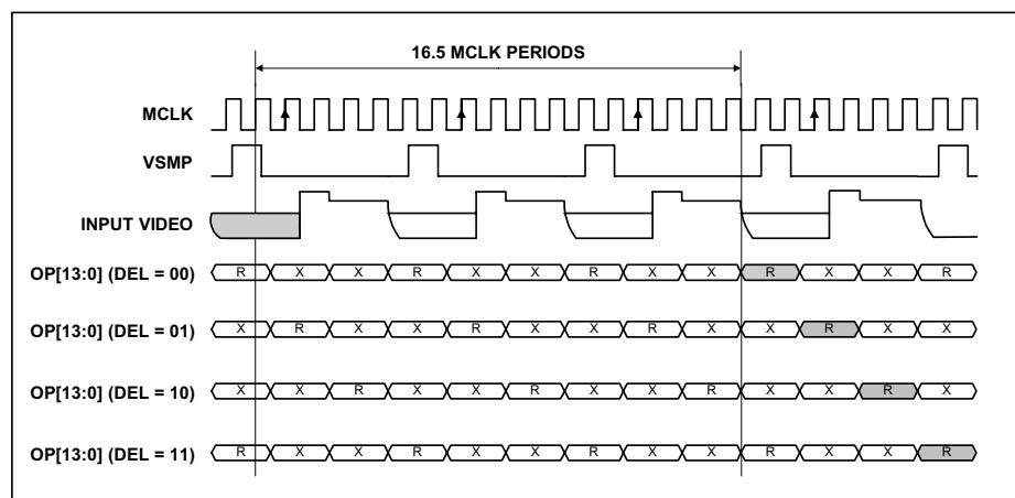
Figure 22 Mode 2 Operation
