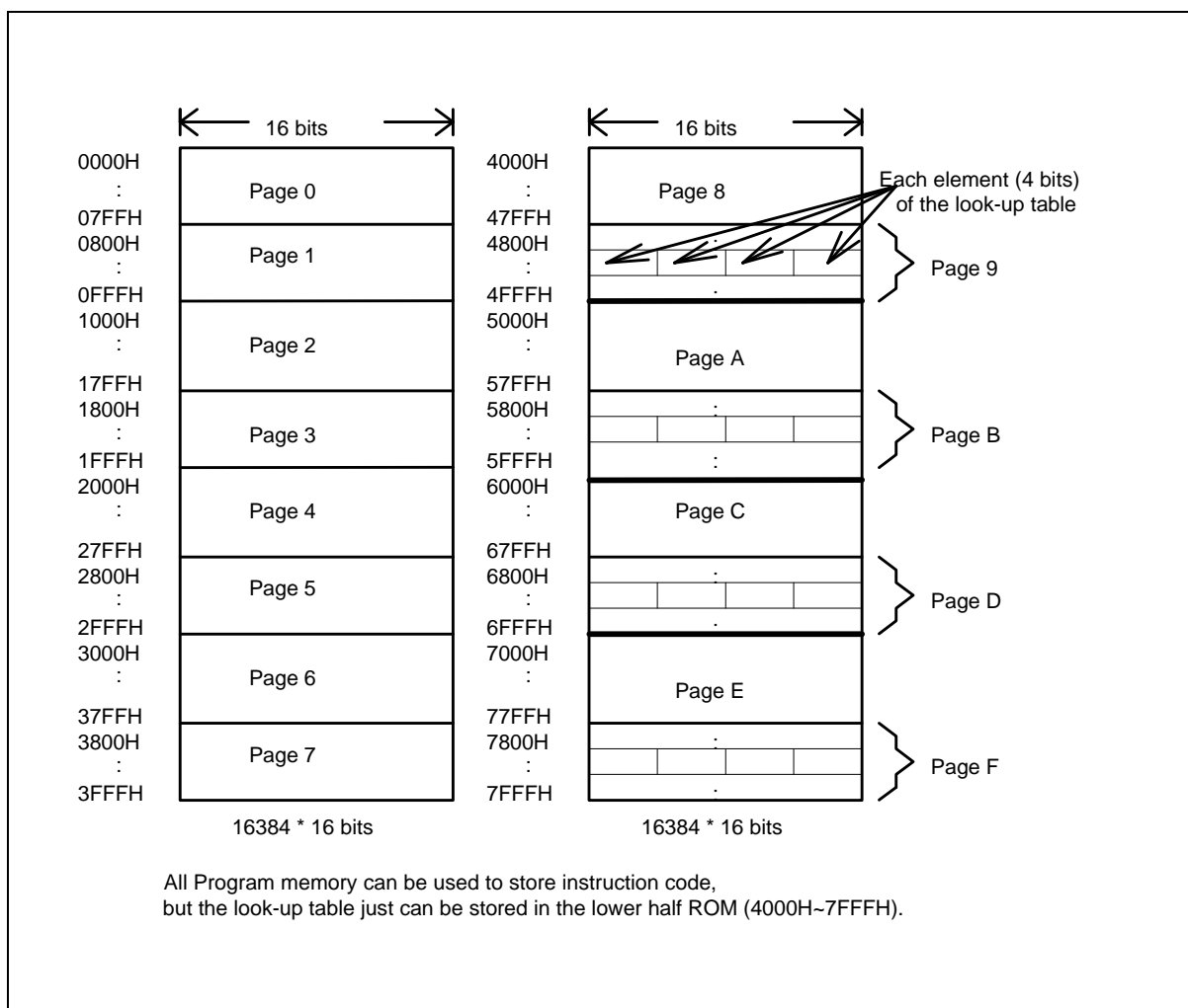
Figure 5-1 Program Memory Organization
