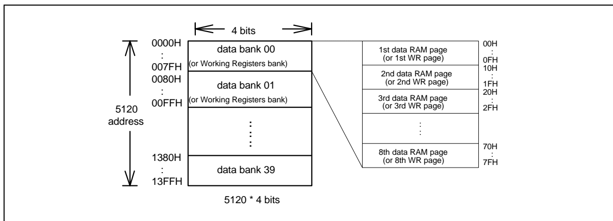
Figure 5-2 Data Memory Organization
