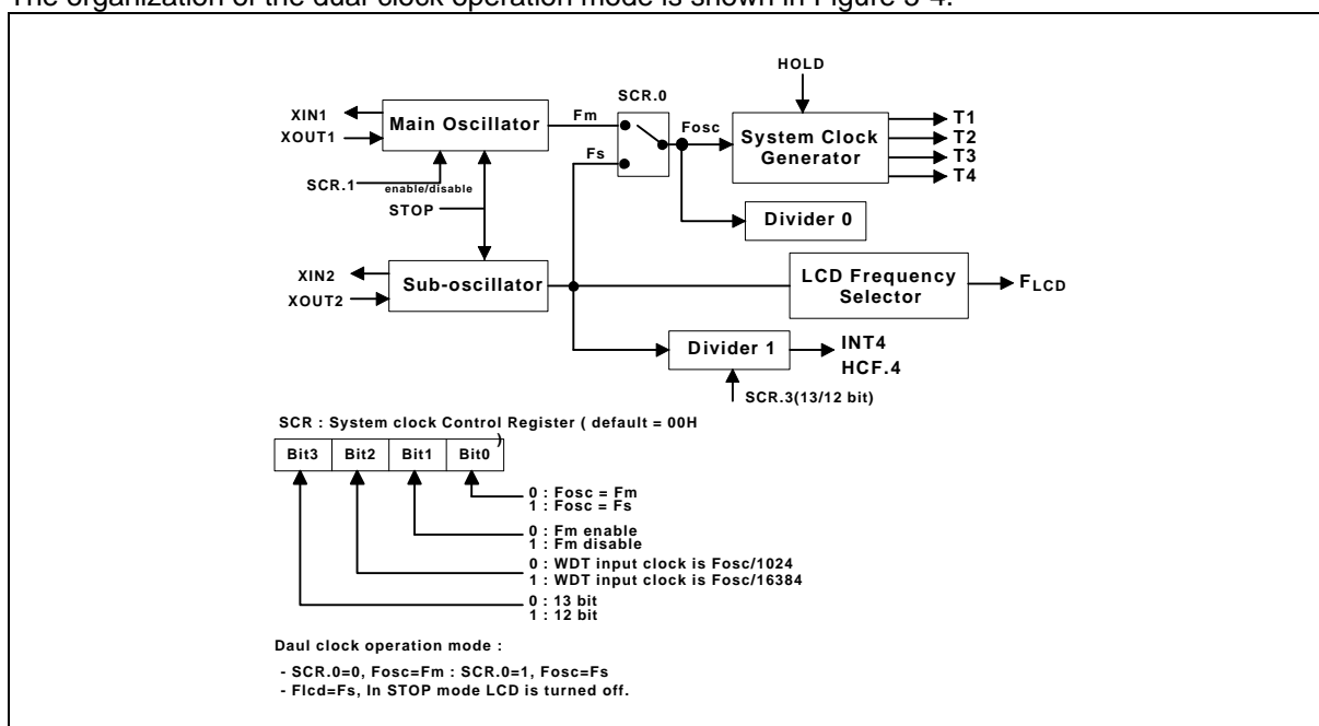
Figure 5-4 Organization of the dual-clock operation mode
