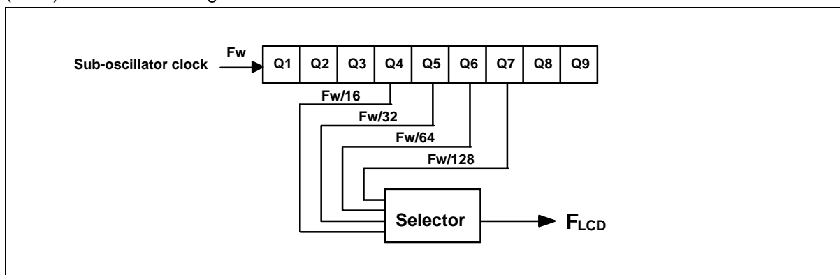
Figure 5-17 LCD alternating frequency (FLCD) circuit diagram
