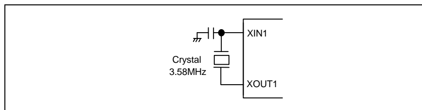
Figure 5-3 System clock oscillator Configuration
