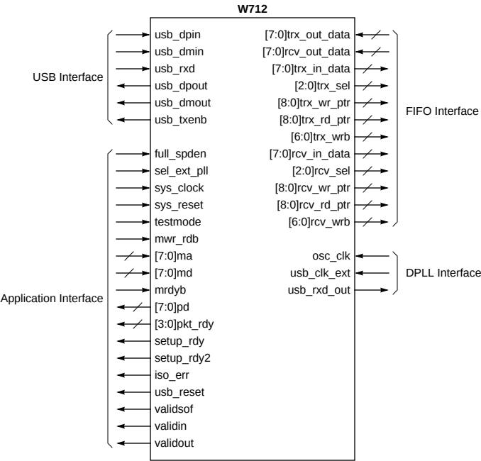
Figure 1. Logic Symbol
