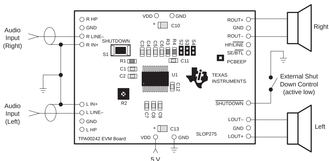
Figure 3–9. TPA0242 EVM Connected for Stereo BTL Output
