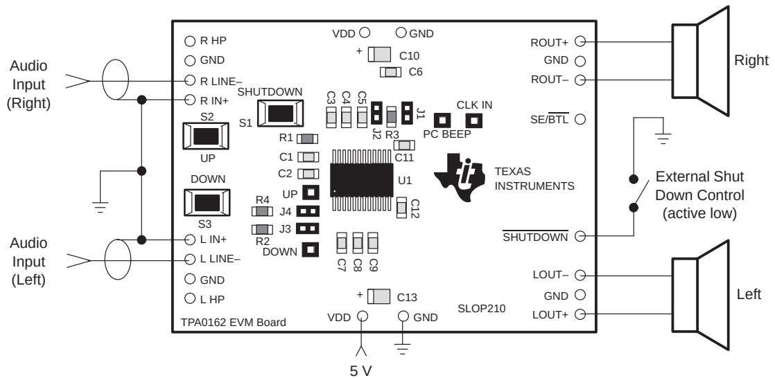
Figure 3–9. TPA0162 EVM Connected for Stereo BTL Output
