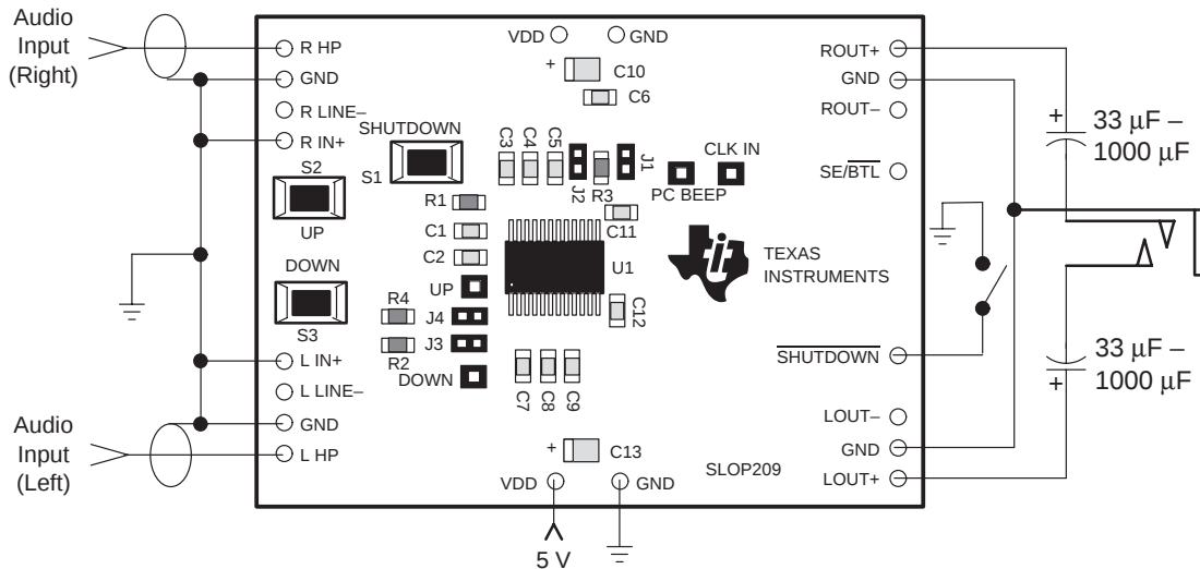
Figure 3–10. TPA0152 EVM Connected for Stereo Single-Ended Output
