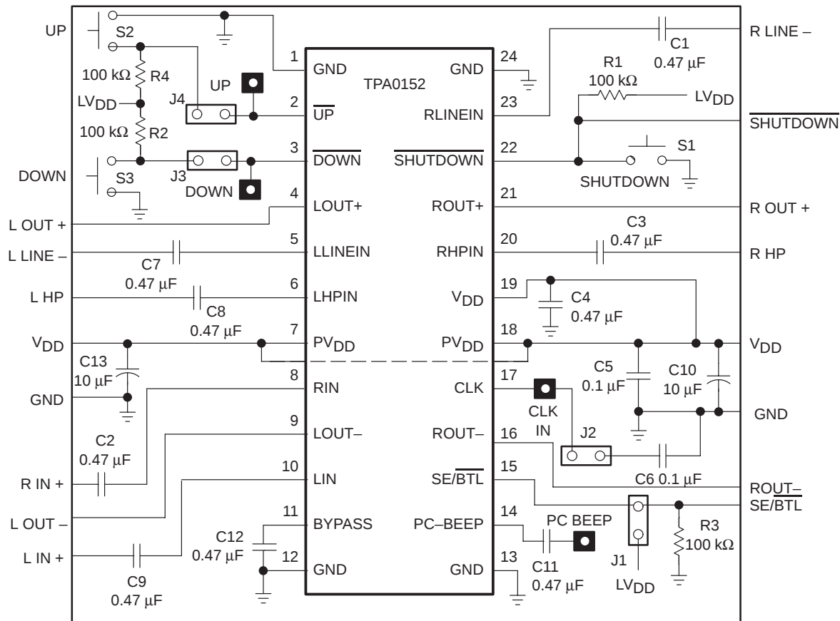
Figure 3–3. TPA0152 EVM Schematic Diagram
