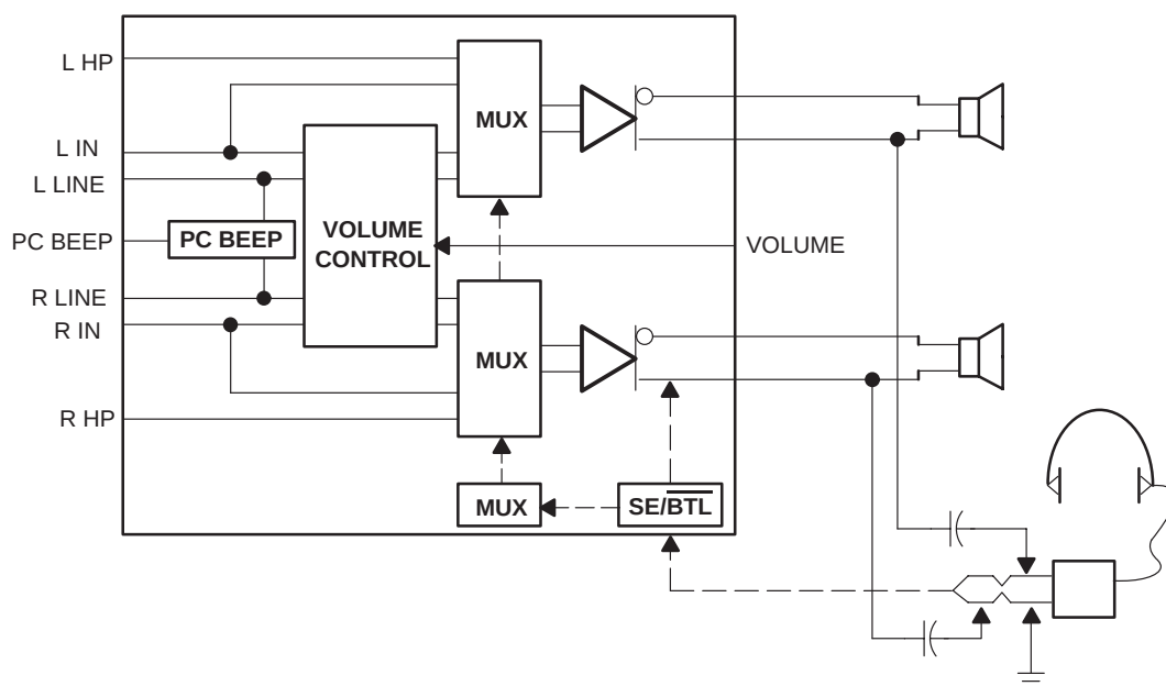
Figure 3–4. TPA0152 Amplifier IC
