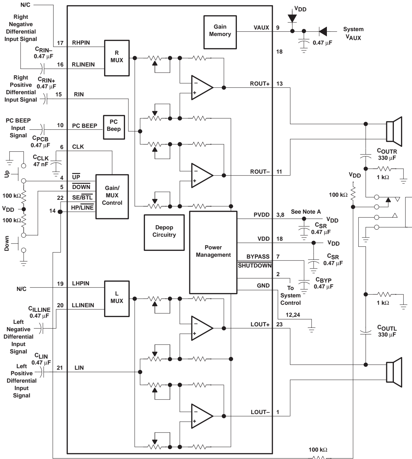
Figure 31. Typical TPA0252 Application Circuit Using Differential Inputs
