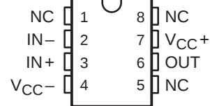
LM107 . . . JG PACKAGE LM207, LM307 . . . D OR P PACKAGE (TOP VIEW)
