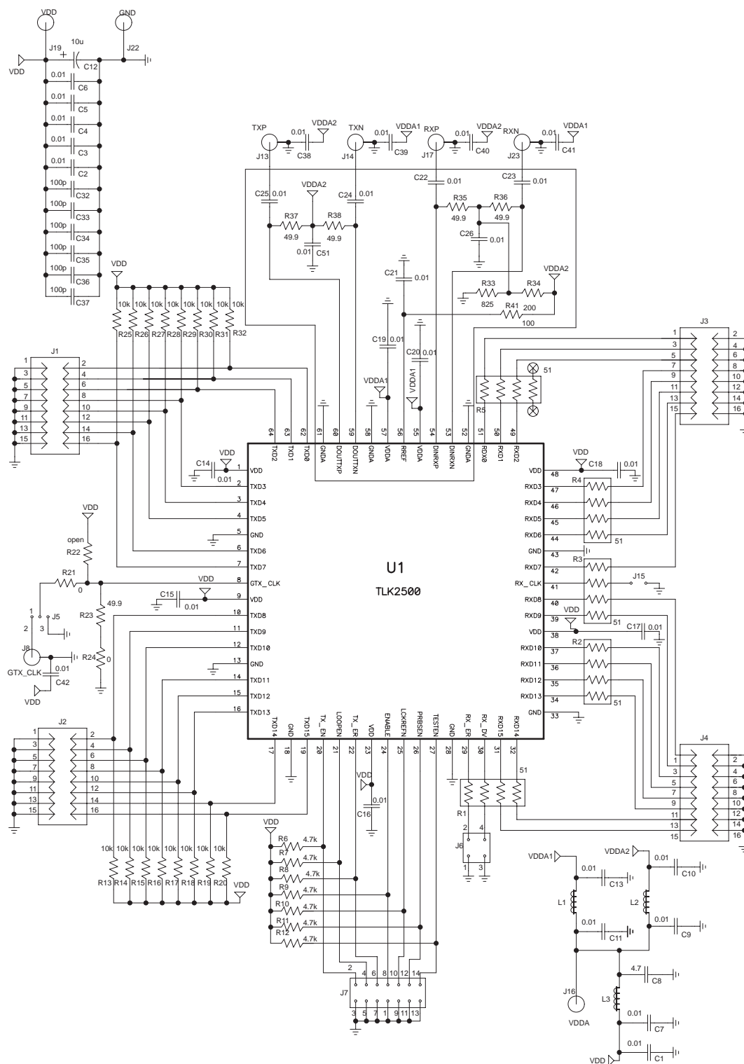
Figure A–1. TLK2500 EVM Transceiver Schematic
