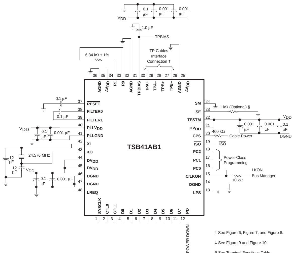
Figure 5. External Component Connections (PHP)
