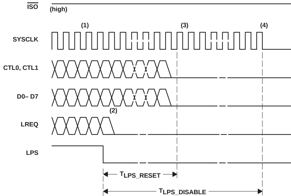
Figure 26. Interface Disable, \overline{\text{ISO}} High
