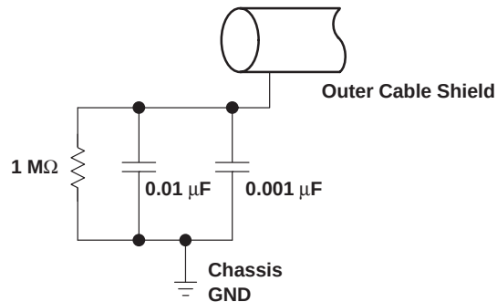
Figure 7. Compliant DC Isolated Outer Shield Termination
