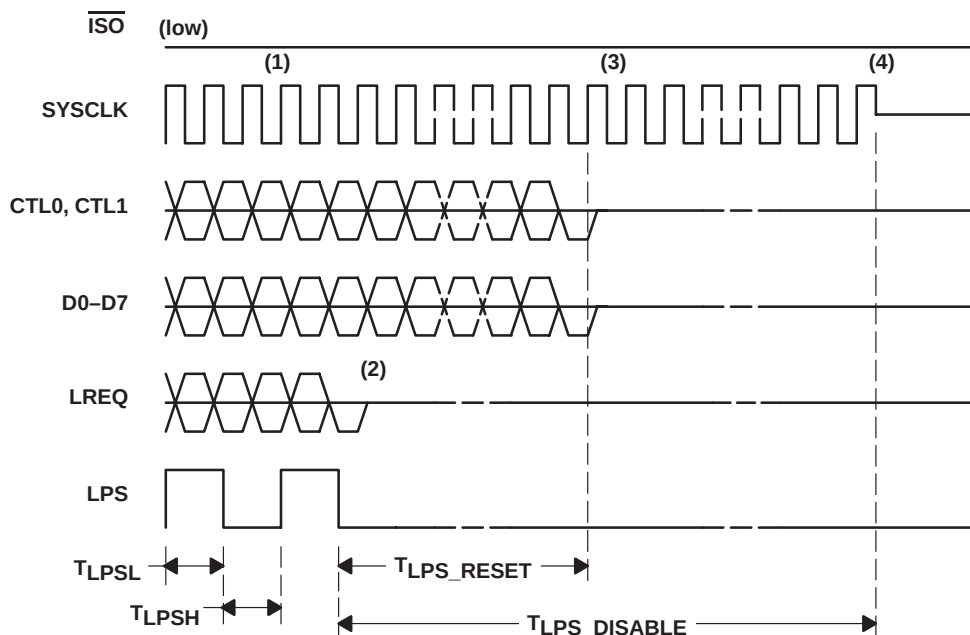
Figure 25. Interface Disable, \overline{ISO} Low
