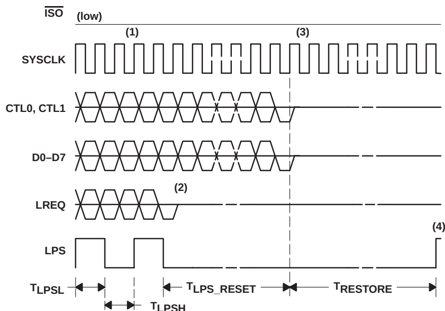
Figure 23. Interface Reset, \overline{\text{ISO}} Low
