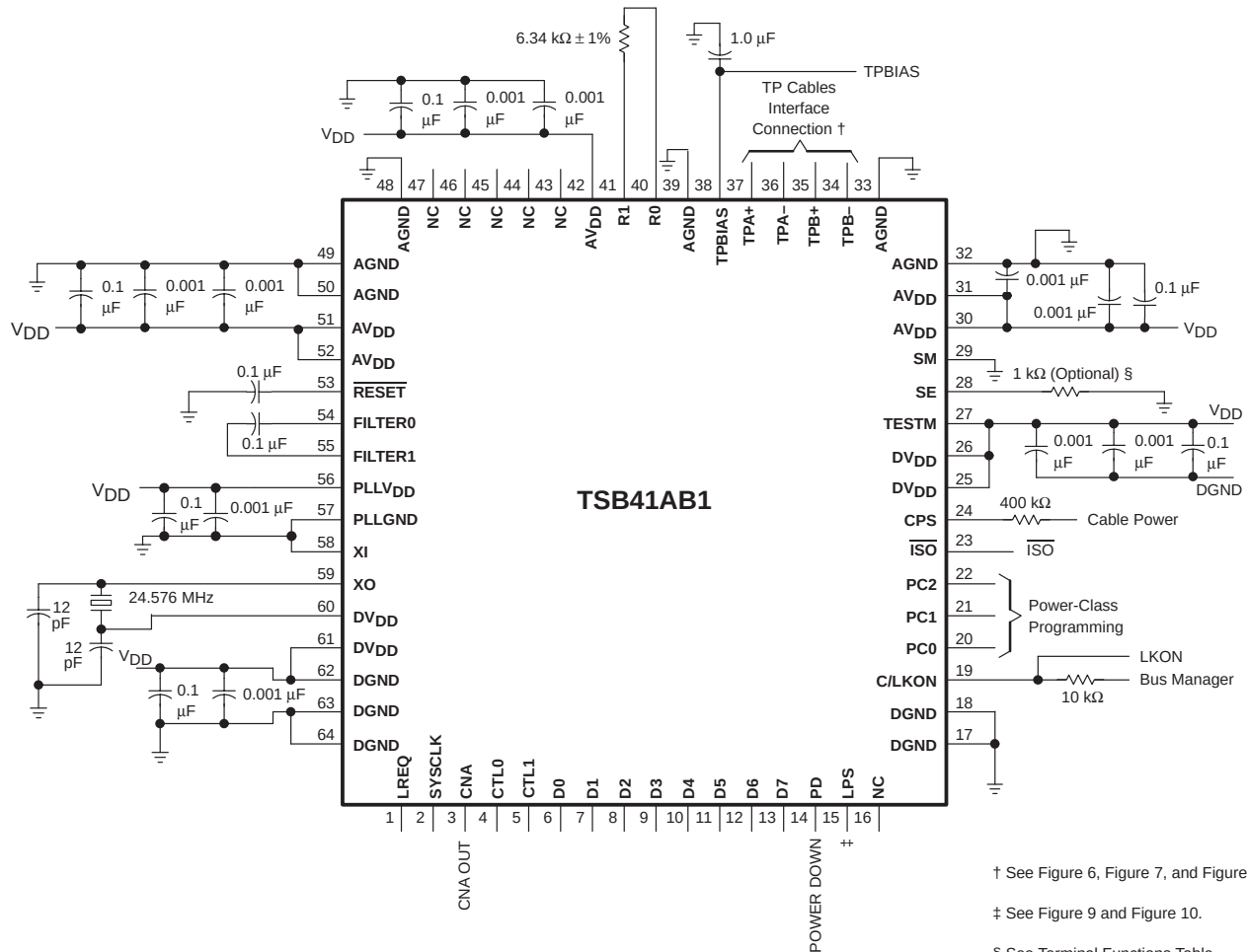
Figure 4. External Component Connections (PAP)
