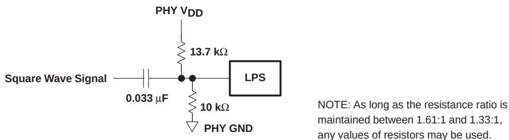
Figure 10. Isolated Circuit Connection for LPS
