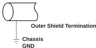
Figure 8. Non-Isolated Outer Shield Termination
