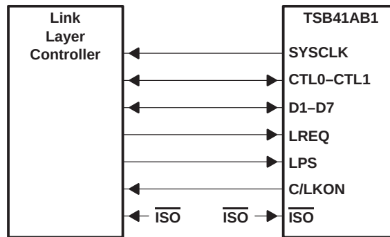
Figure 14. PHY-LLC Interface
