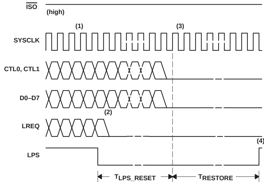
Figure 24. Interface Reset, \overline{ISO} High
