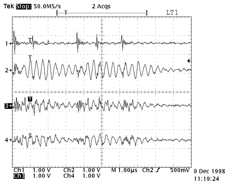
Figure 4. Fluorescent Light Switched On/Off (Scope Time Base at 1 µs) †
