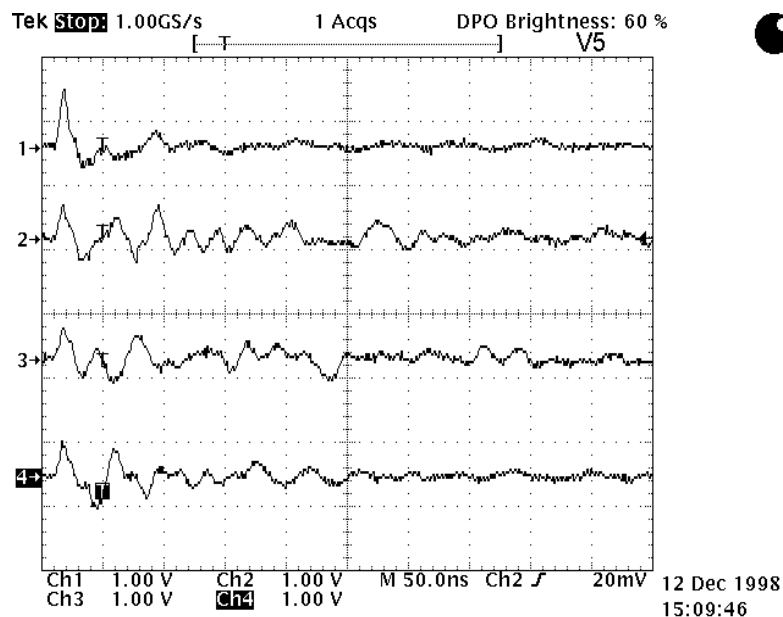
Figure 10. Cables Tied to Chassis Ground on a VLSI Logic Tester and Powered On/Off
