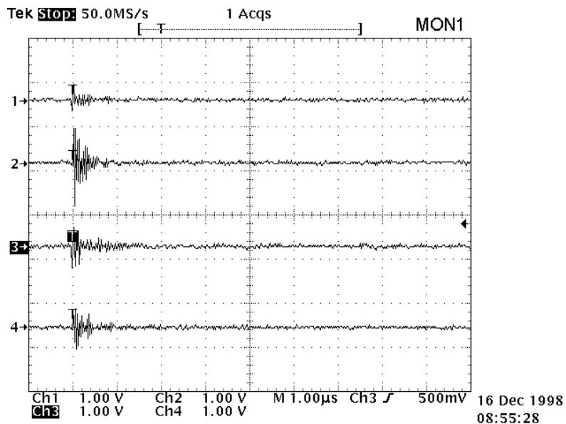
Figure 2. PC Monitor Power Switched On/Off (Scope Time Base at 1 \mu s) †
