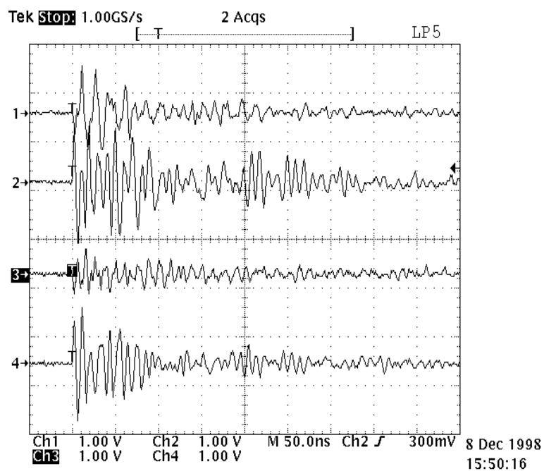
Figure 9. 208 VAC Power Line in Conduit (Scope Time Base at 50 ns) †
