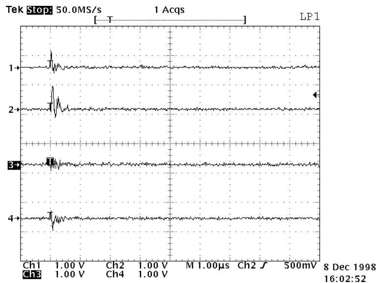
Figure 8. 208 VAC Power Line in Conduit (Scope Time Base at 1 µs) †
