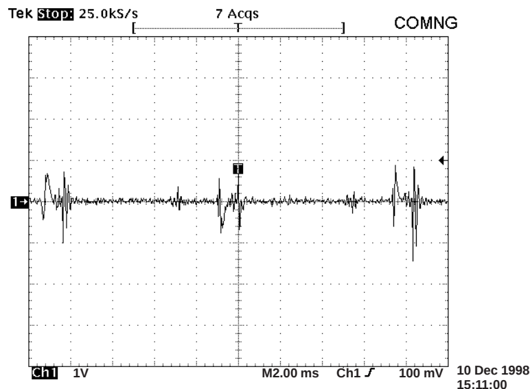
Figure 12. Common Mode Noise From Neutral to Ground
