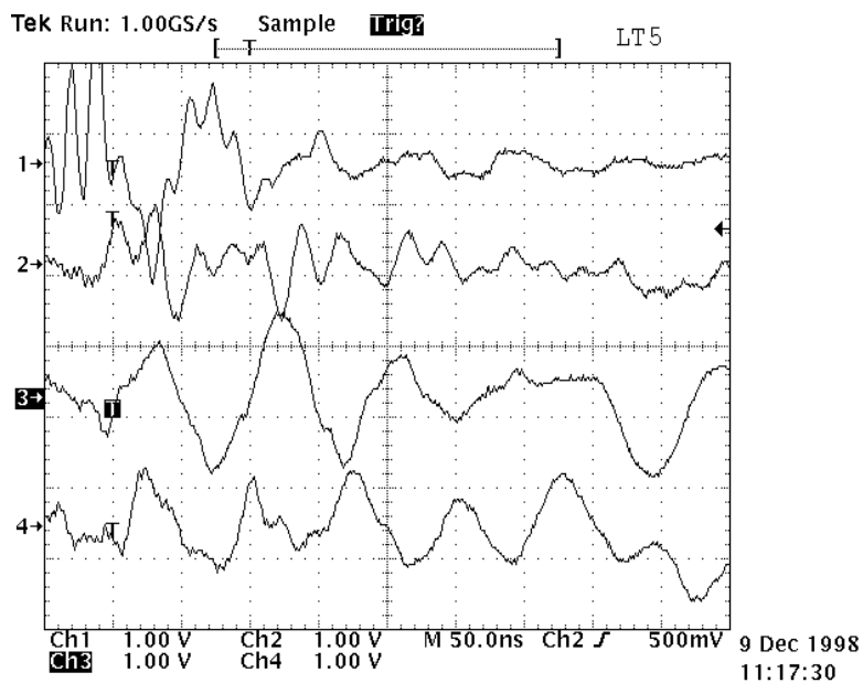
Figure 5. Fluorescent Light Switched On/Off (Scope Time Base at 50 ns) †
