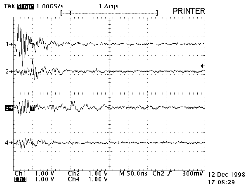
Figure 11. Cables Connected to a Networked Laser Printer Ground While Printing
