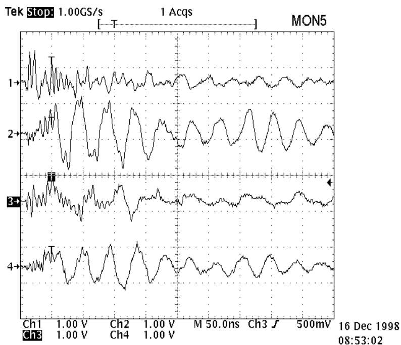
Figure 3. PC Monitor Power Switched On/Off (Scope Time Base at 50 ns) †
