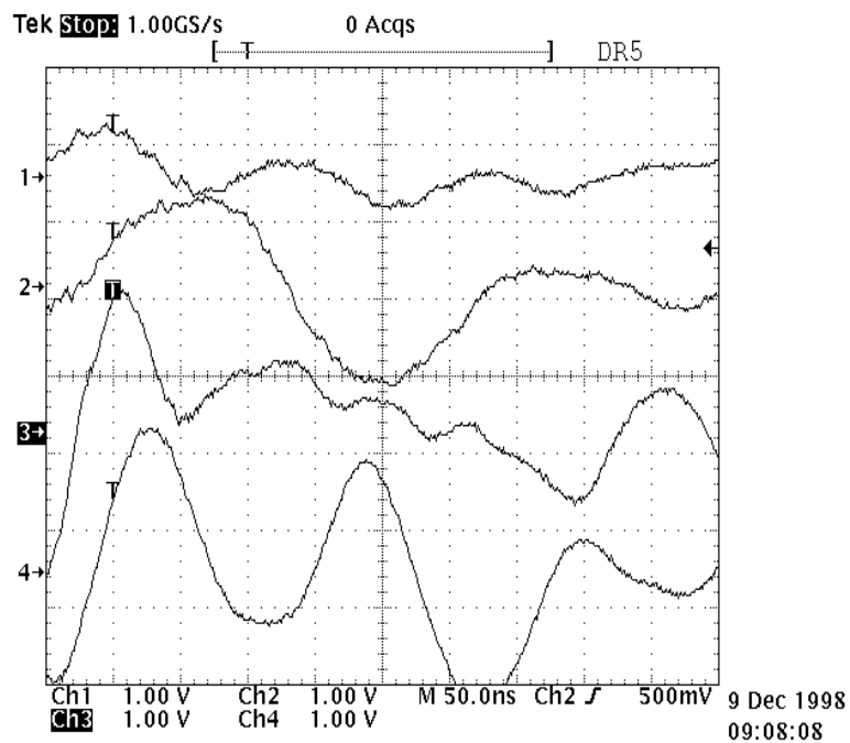
Figure 7. 110-V Drill Press Motor (Scope Time Base at 50 ns) †
