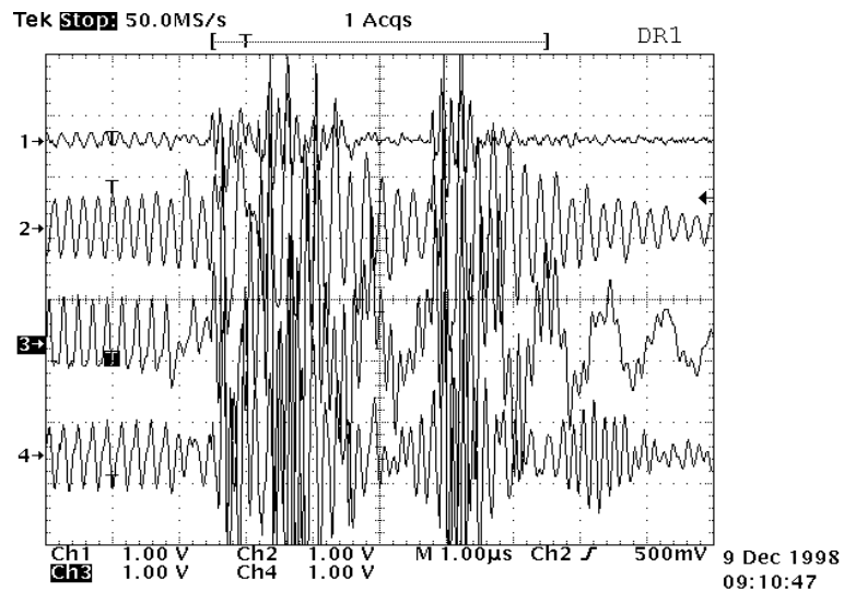
Figure 6. 110-V Drill Press Motor (Scope Time Base at 1 µs) †
