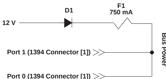
Figure 1. Fuse Placement
