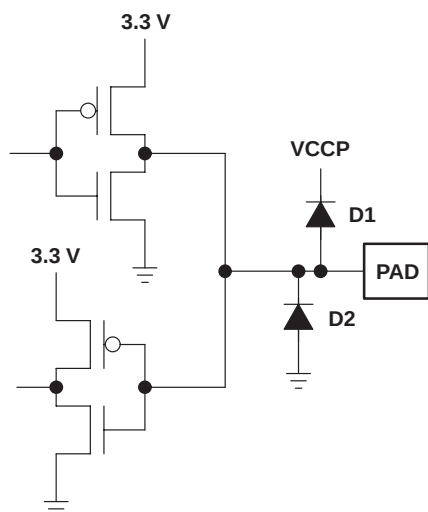
Figure 3. Clamping Voltage
