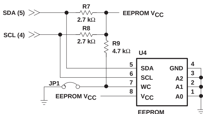
Figure 6. Serial EEPROM
