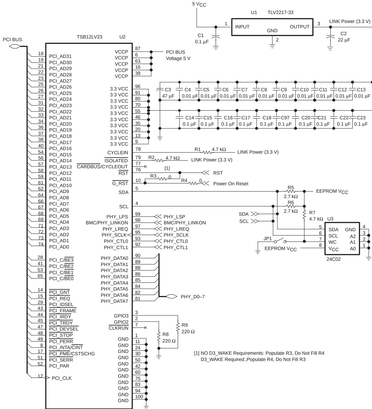
Figure 7. TSB12LV23 Schematic
