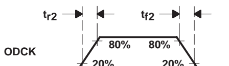
Figure 2. Rise and Fall Time of ODClock
