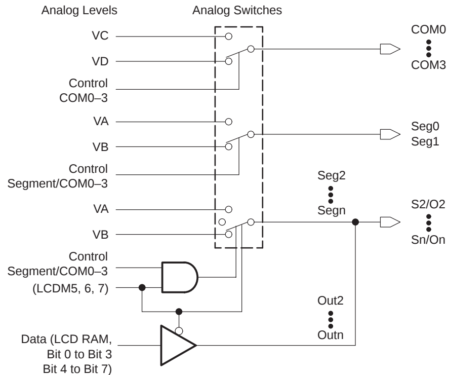
Figure 14–7. Schematic of LCD Output
