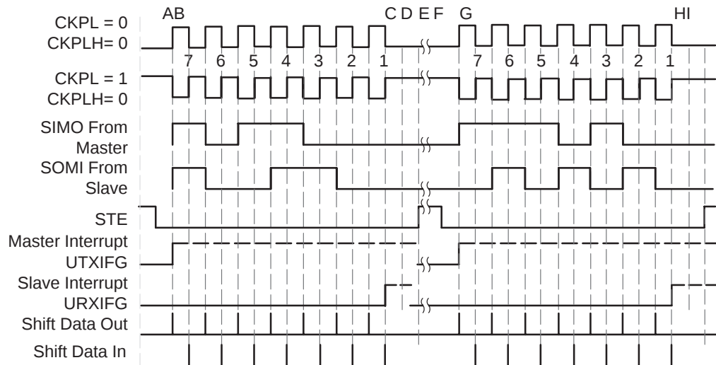
Figure 13–4. Serial Synchronous Data Transfer
