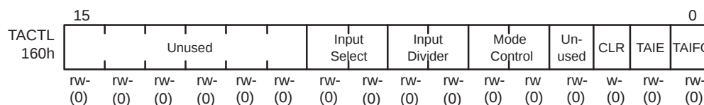
Figure 11–27. Timer_A Control Register TACTL
