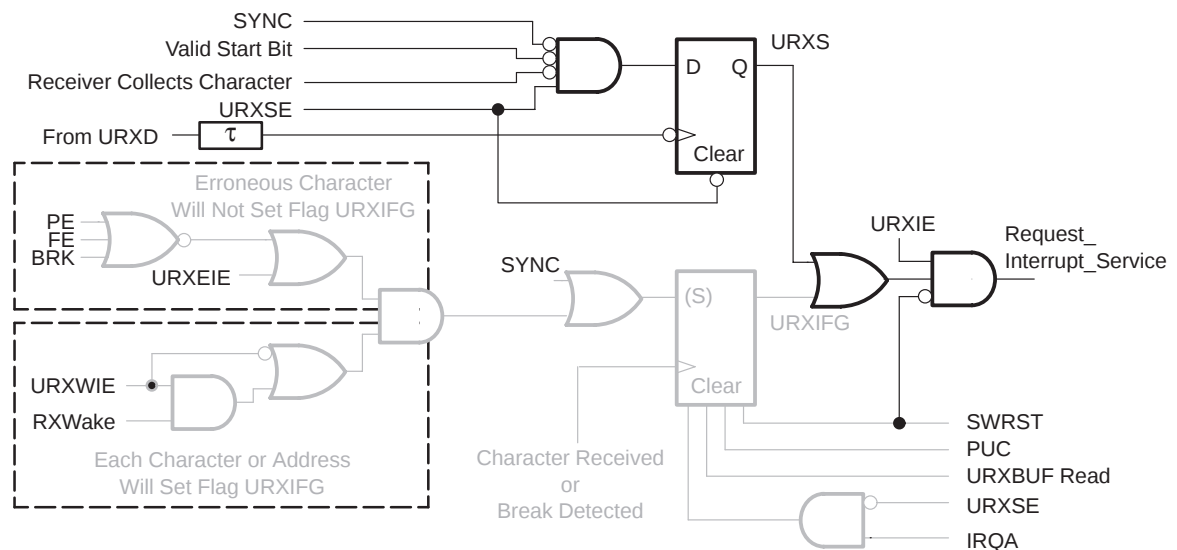
Figure 12–23. Receive-Start Conditions
