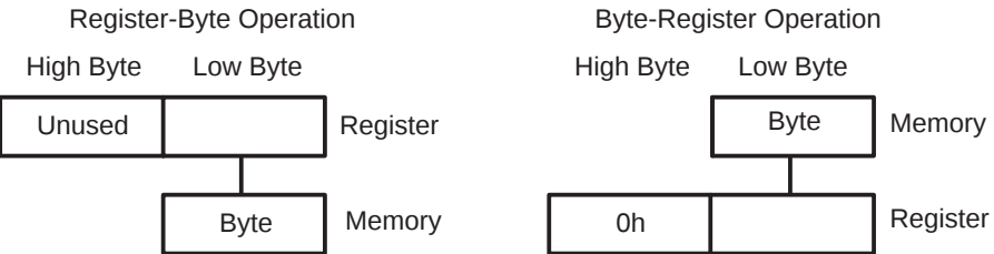
Figure 4–6. Register-Byte/Byte-Register Operations
