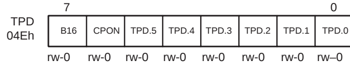
Figure 9–6. Timer/Port Data Register
