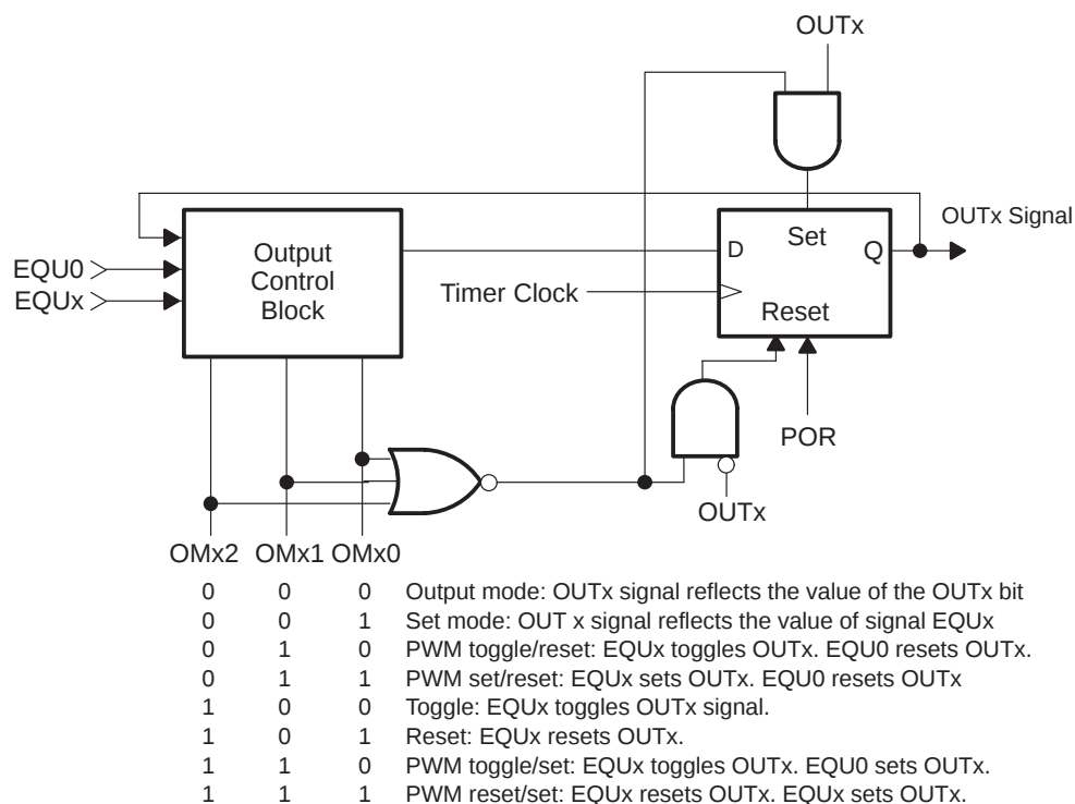
Figure 11–22. Output Unit
