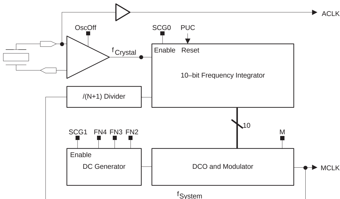
Figure 7–1. Frequency-Locked Loop
