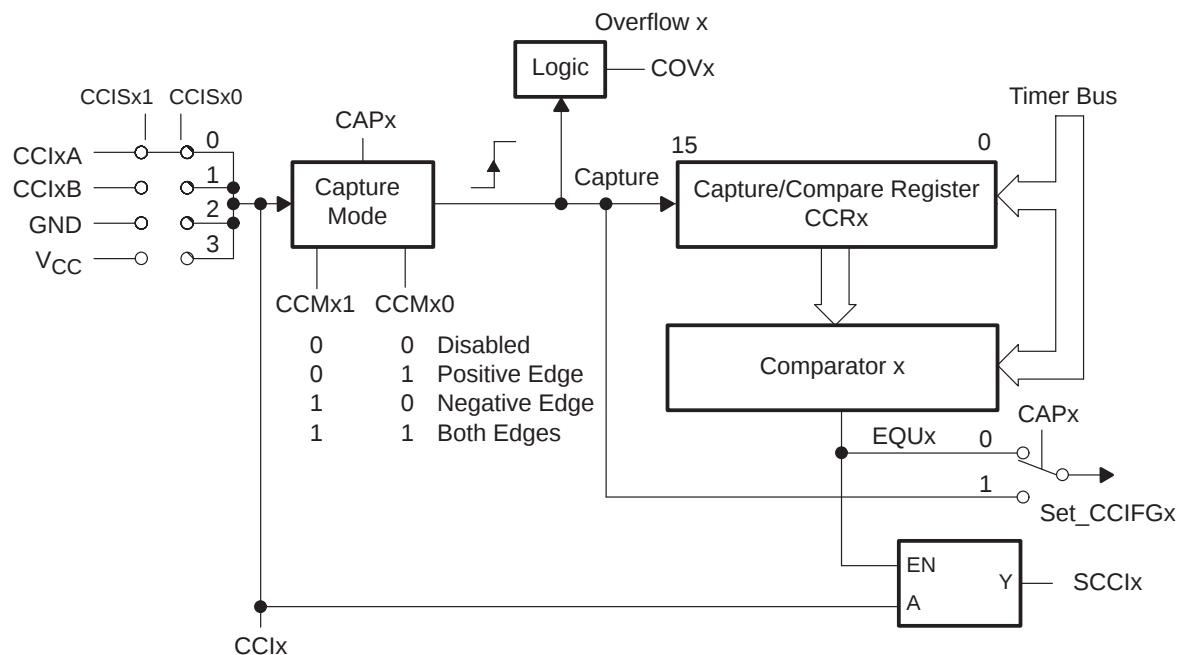
Figure 11–17. Capture/Compare Blocks
