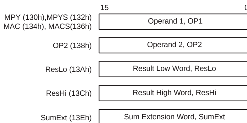
Figure 6–3. Registers of the Hardware Multiplier
