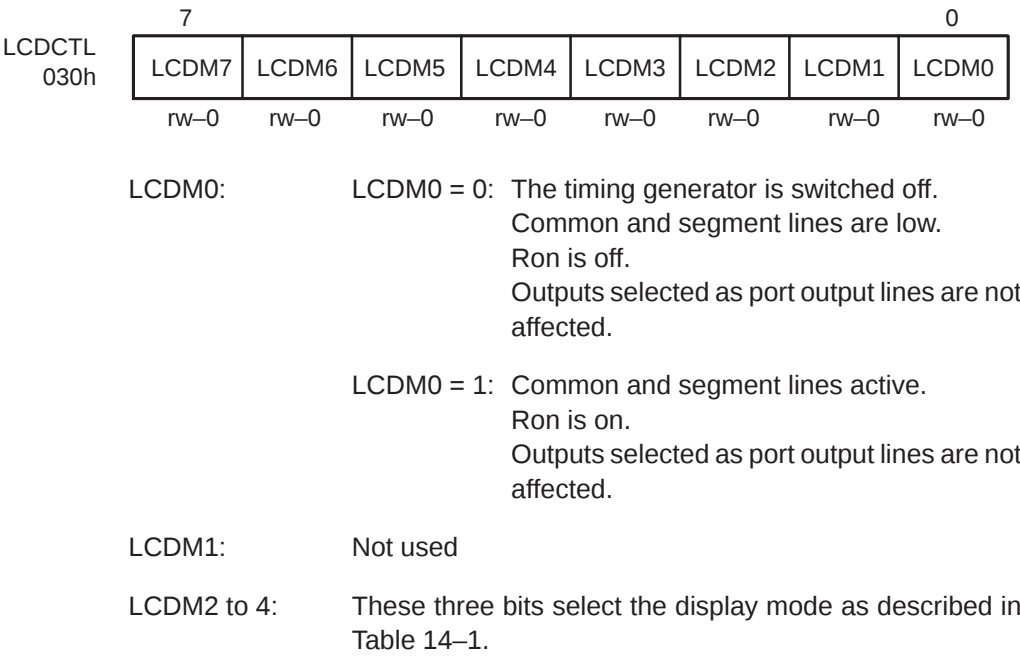
Figure 14–11. LCD Control and Mode Register
