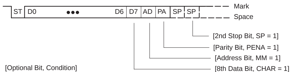
Figure 12–3. Asynchronous Frame Format
