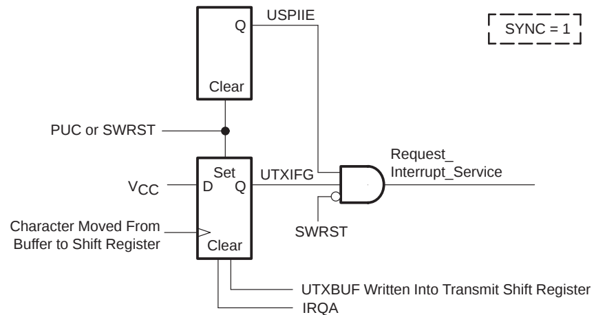
Figure 13–14. Transmit-Interrupt Operation
