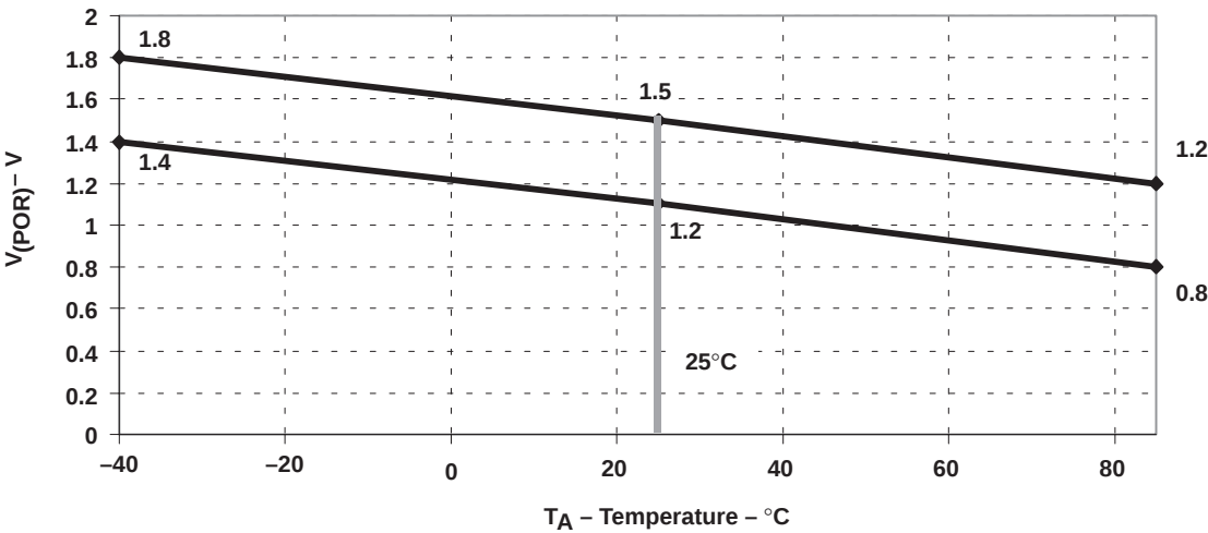
Figure 9. V(POR) vs Temperature
