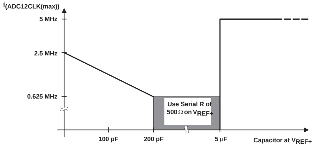
Figure 12. Maximum Frequency f_{\text{ADC12(CLK)}} vs External Capacitor on V_{\text{REF+}}
