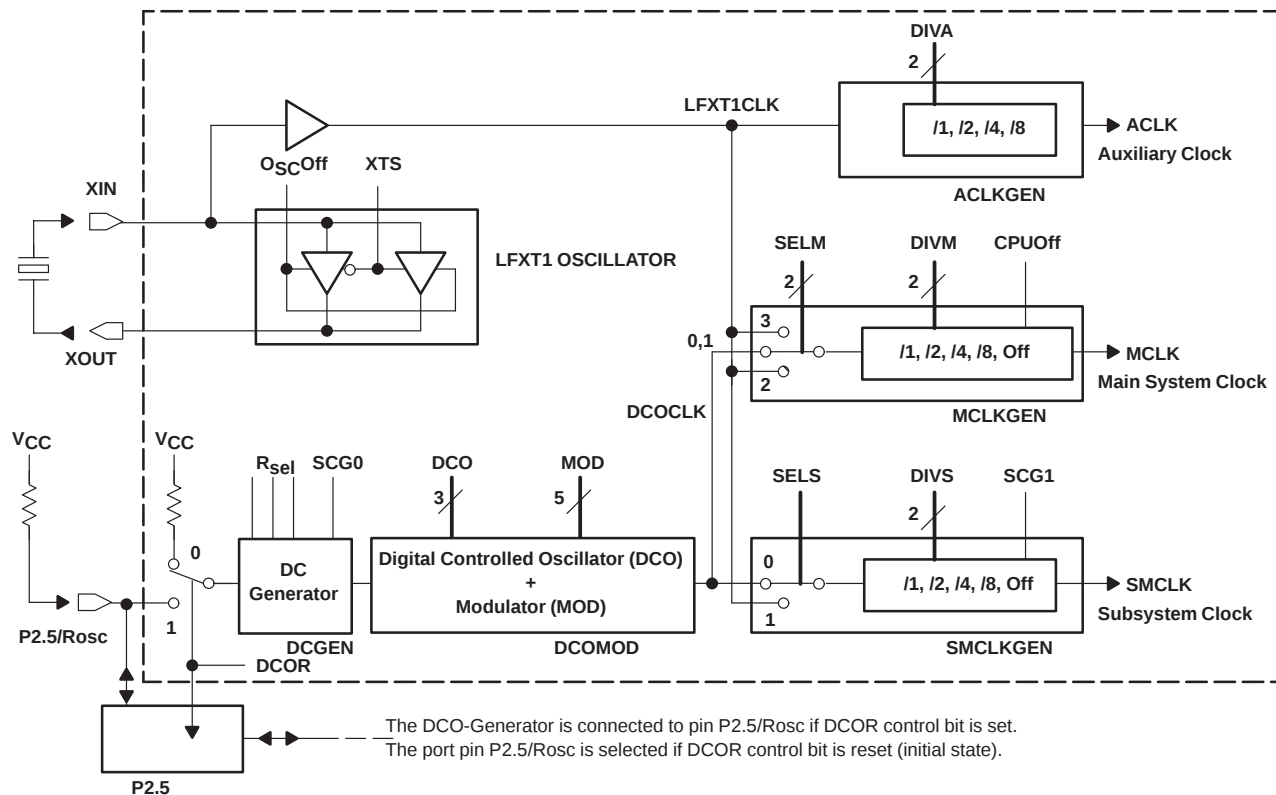
Figure 3. Clock Signals
