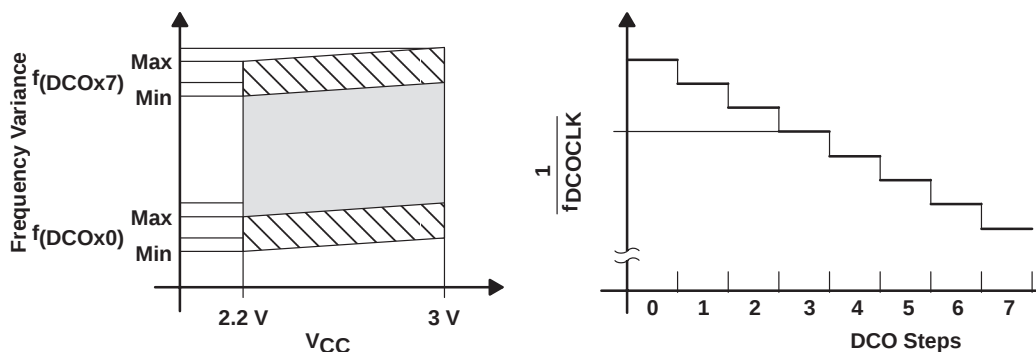
Figure 8. DCO Characteristics
