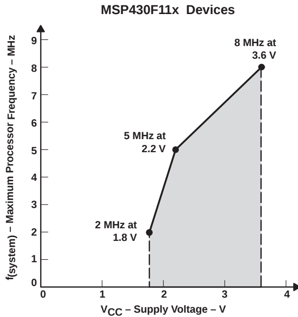
Figure 5. Frequency vs Supply Voltage
