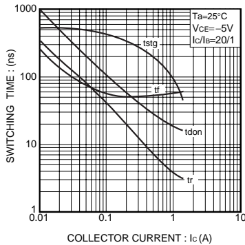
Fig.13 Switching time
