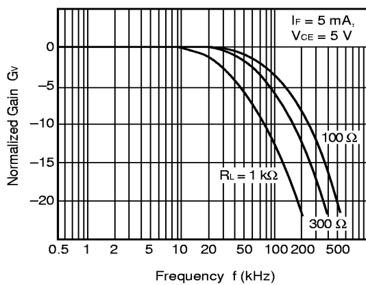
FREQUENCY RESPONSE
