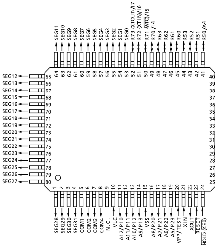
QFP80-P-1420-0.80B
