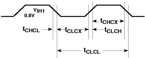
Figure 6. External Clock Drive at XTAL1
