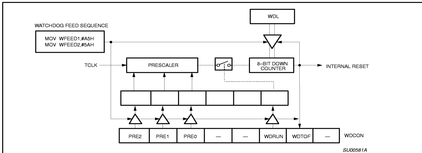
Figure 10. Watchdog Timer in XA-G1/G2/G3
