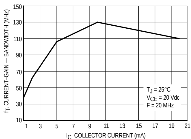
Figure 3. Current-Gain — Bandwidth
