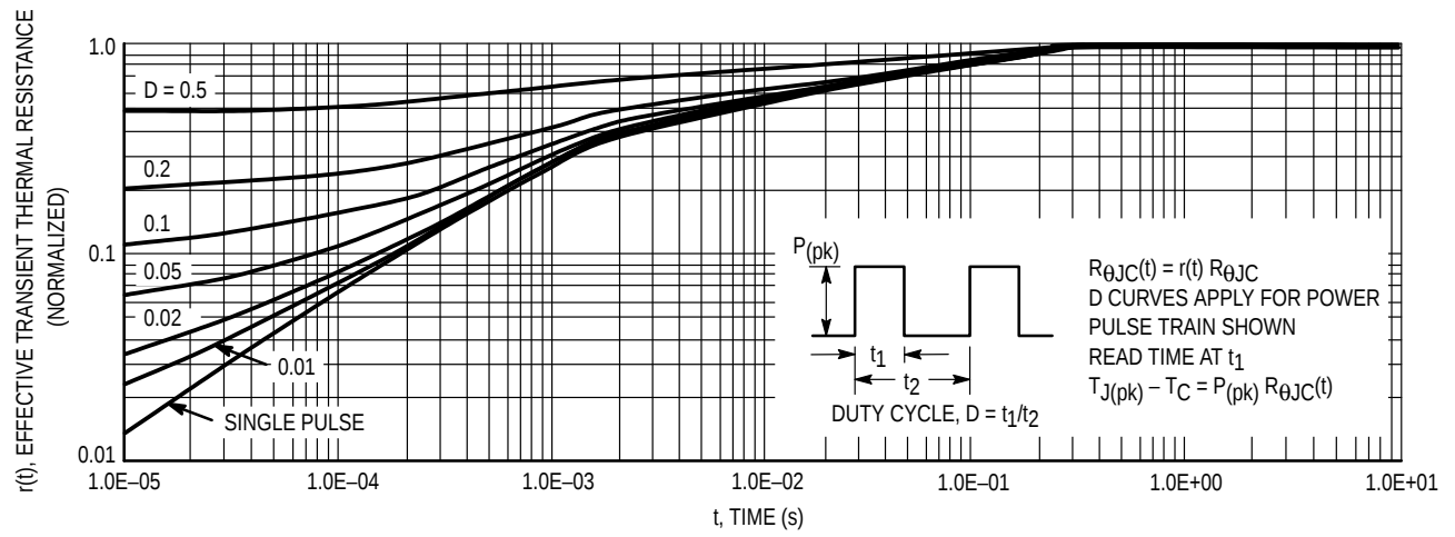
Figure 14. Thermal Response
