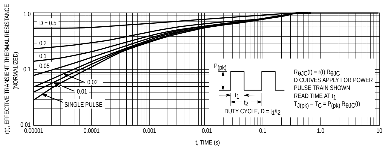
Figure 14. Thermal Response
