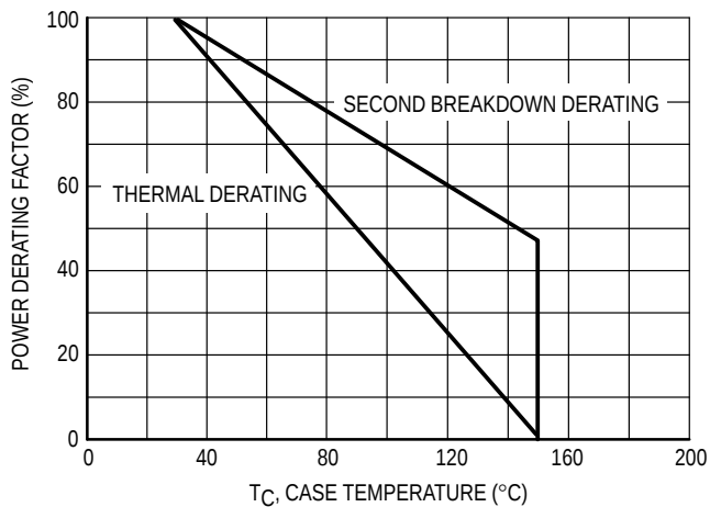
Figure 16. Power Derating
