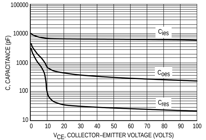
Figure 16. Capacitance Variation
