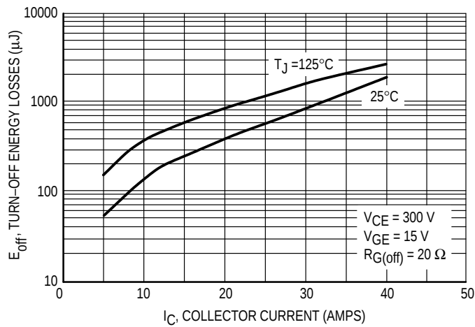
Figure 13. Turn-Off Energy Losses versus Collector Current
