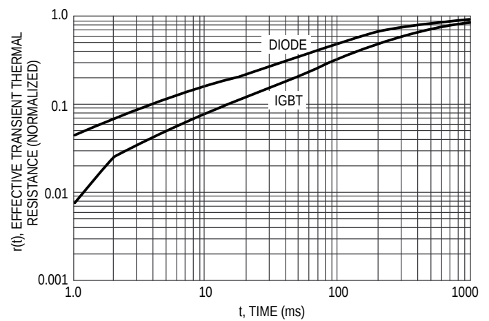
Figure 18. Thermal Response
