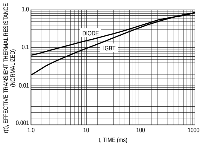
Figure 18. Thermal Response
