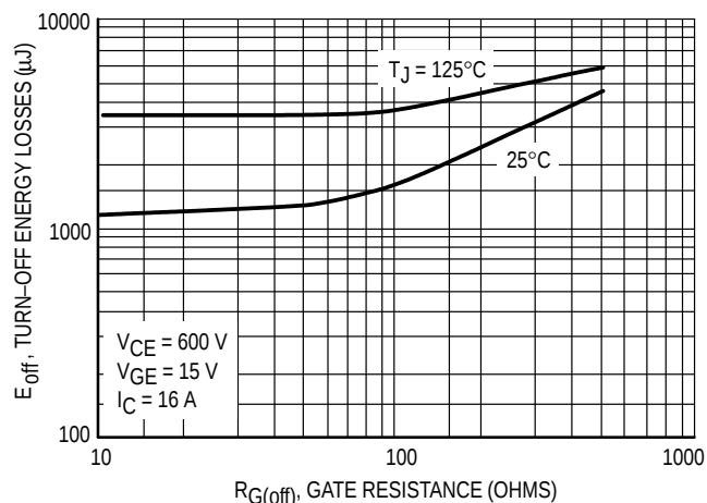
Figure 14. Turn-Off Energy Losses versus Gate Resistance
