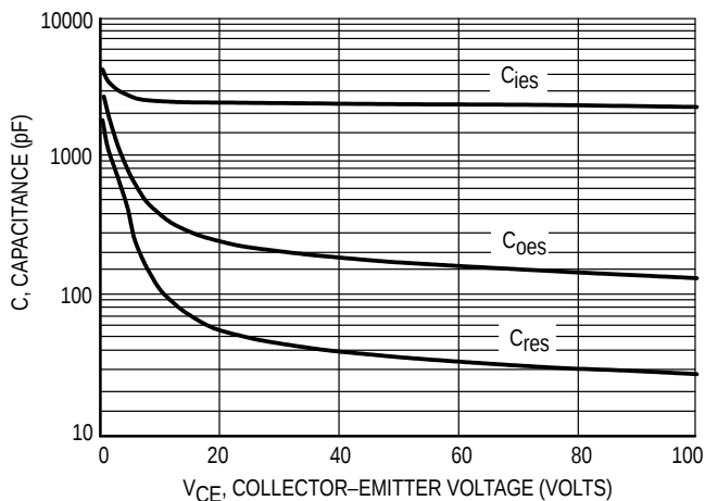
Figure 16. Capacitance Variation
