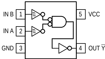
Figure 1. 5-Lead SOT-353 Pinout (Top View)
