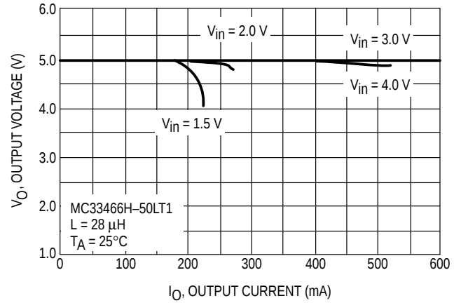
Figure 8. Output Voltage versus Output Current
