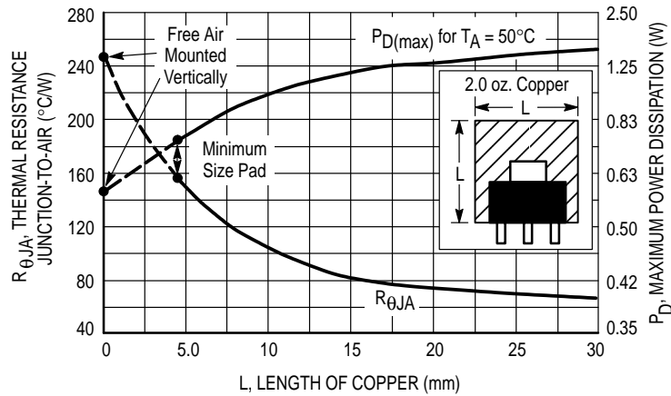
Figure 15. SOT-223 Thermal Resistance and Maximum Power Dissipation versus P.C.B. Copper Length
