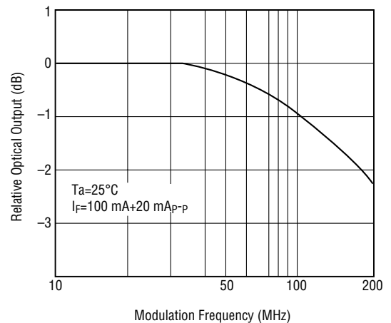
Frequency Response
