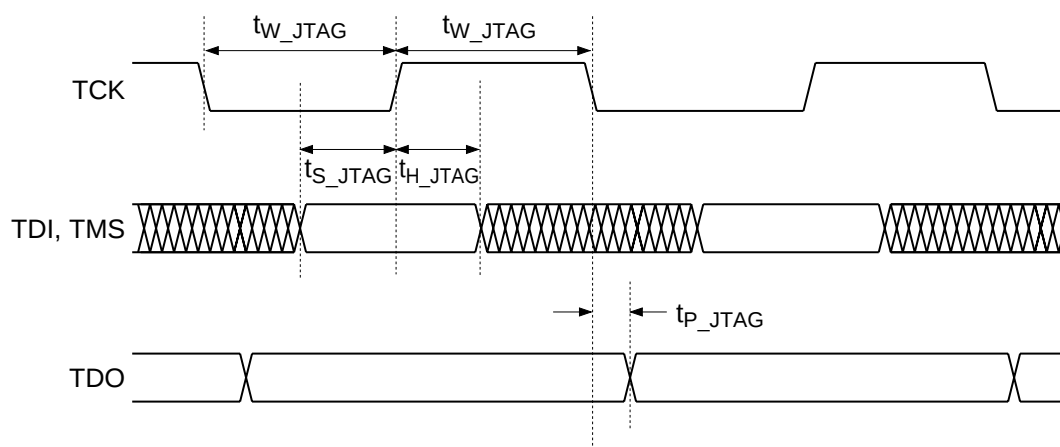
Figure 17 JTAG Timing
