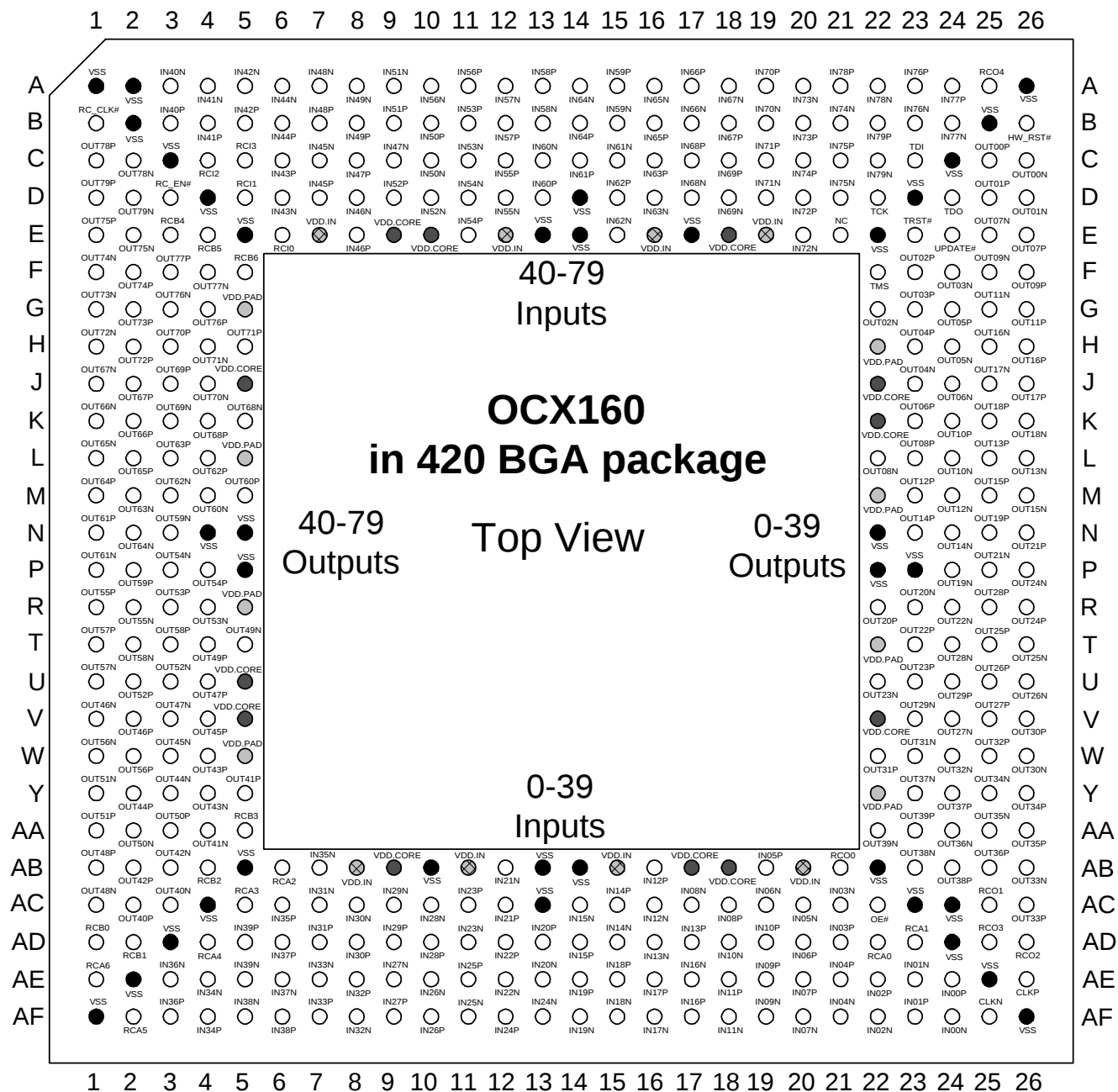
Figure 19 OCX160 Package Pinout
