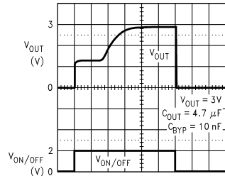
Turn-ON Waveform
