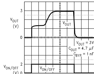
Turn-ON Waveform
