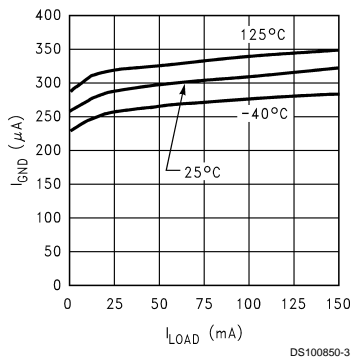
Ground Pin Current vs Load Current over temperature (one LDO on)
