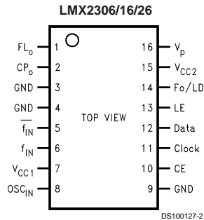
16-Lead (0.173" Wide) Thin Shrink Small Outline Package(TM)
