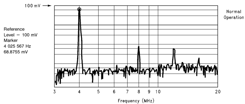
Output Signal Isolation in Disable Mode
