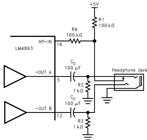
FIGURE 3. Headphone Circuit
