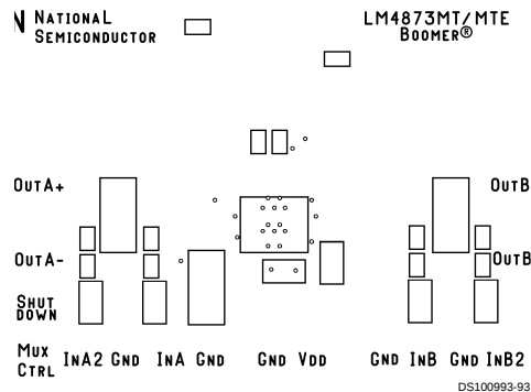
Silk Screen Layer
