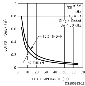
Output Power vs Load Impedance
