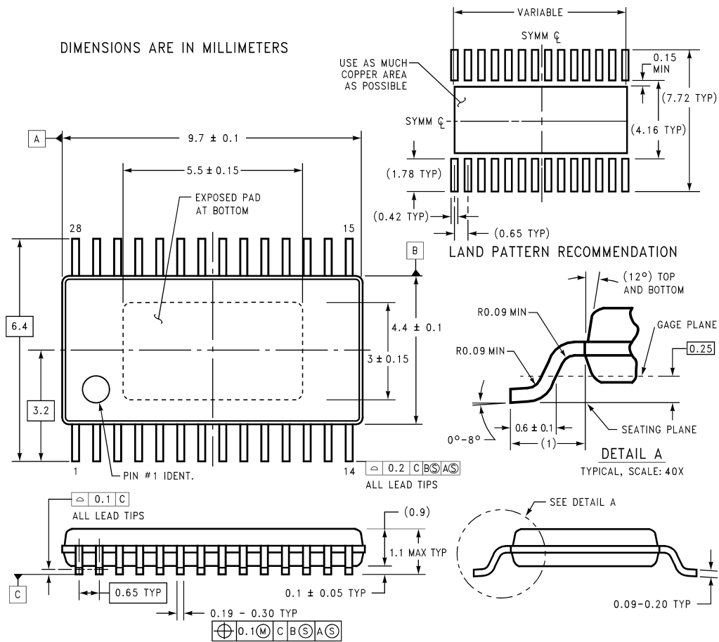
28-Lead Exposed-DAP Thin Small Shrink Outline Package, EIAJ, Type I Order Number LM4873MTE-1 NS Package Number MXA28A
