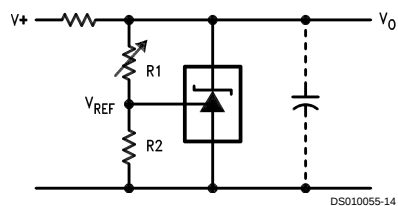
Shunt Regulator
