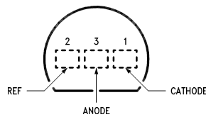
TO-92: Plastic Package
