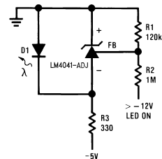
FIGURE 5. Voltage Level Detector
