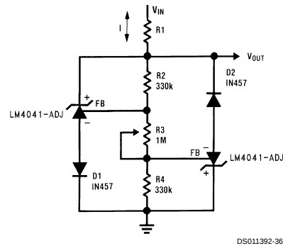
FIGURE 9. Bidirectional Adjustable Clamp ±2.4V to ±6V
