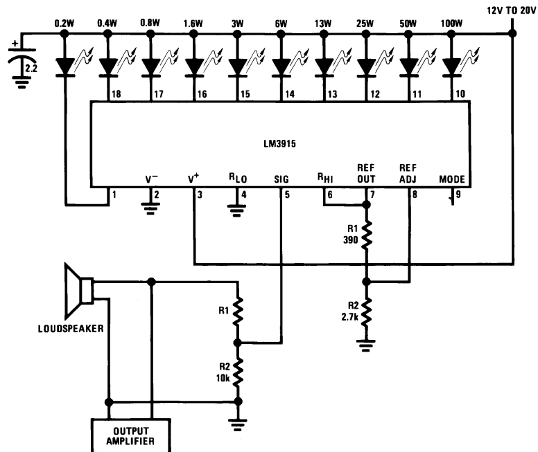
Audio Power Meter
