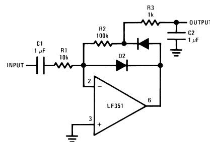
FIGURE 1. Half-Wave Peak Detector
