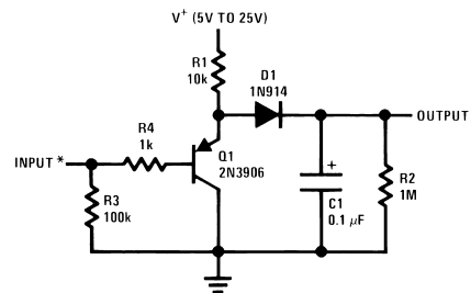
FIGURE 1. Half-Wave Peak Detector
