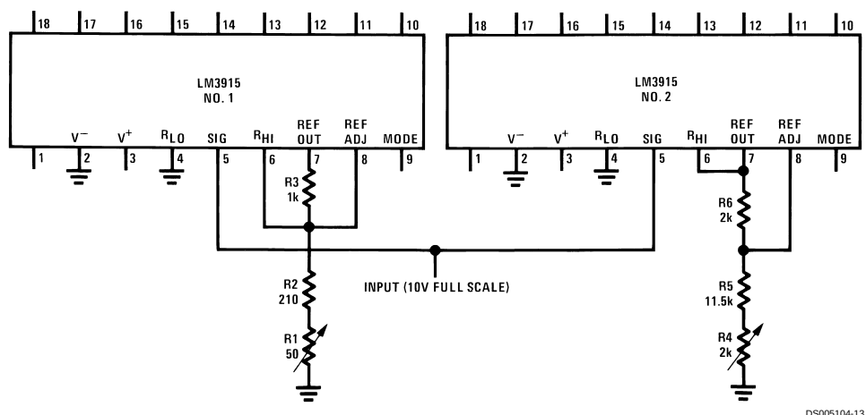
FIGURE 5. Low Cost Circuit for 60 dB Display
