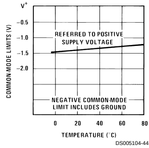
Common-Mode Limits
