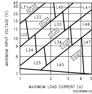
FIGURE 4. LM2678-5.0
