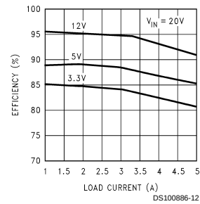
Efficiency vs I_{LOAD}
