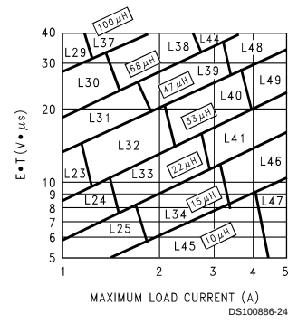
FIGURE 6. LM2678-ADJ
