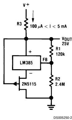
25V Low Current Shunt Regulator
