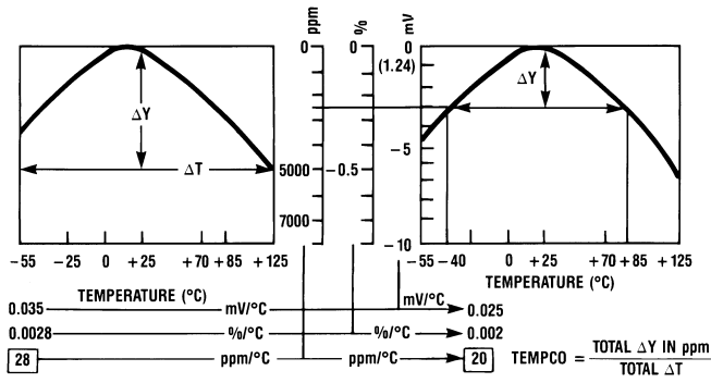
Temperature Coefficient Typical LM185
