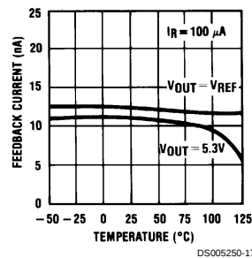
Feedback Current
