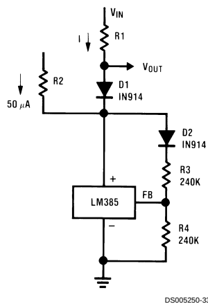
Fast Positive Clamp 2.4V + \Delta V_{D1}
