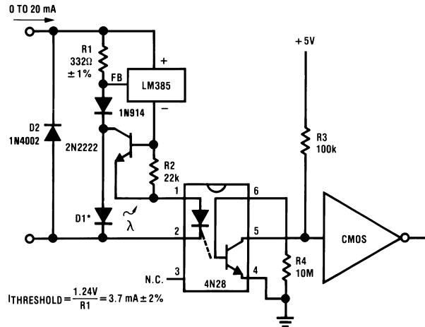
Precision Floating Current Detector
