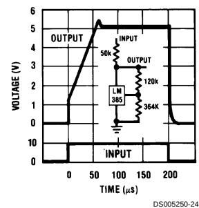
Response Time
