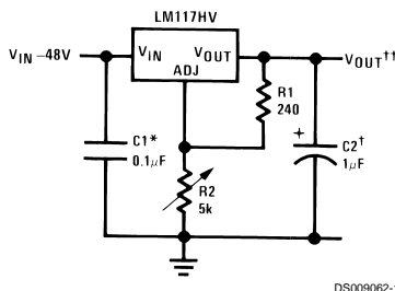
1.2V-45V Adjustable Regulator
