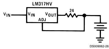
50 mA Constant Current Battery Charger
