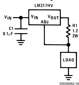
1A Current Regulator
