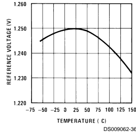
Temperature Stability
